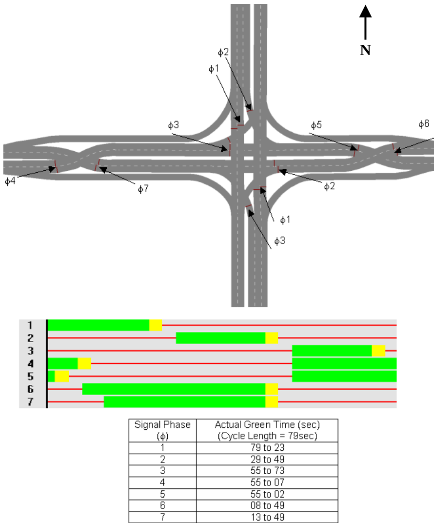
FIGURE 5 Signal setting for DXI.
